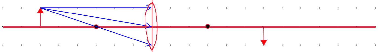
Object at 6 cm, focal length +3 cm.
