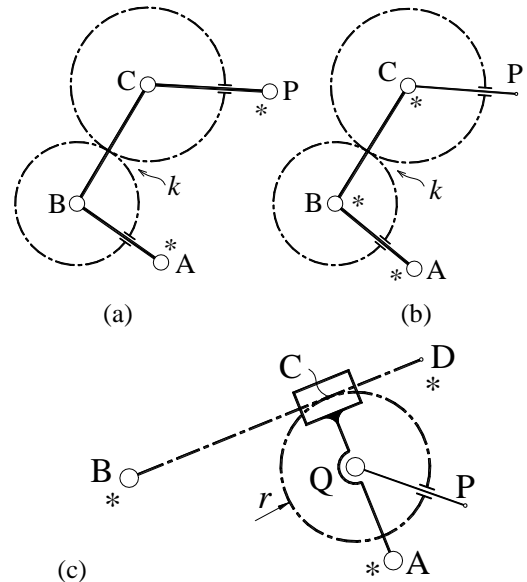
Figure 11: Geared modules available as LibAssur subroutines.
