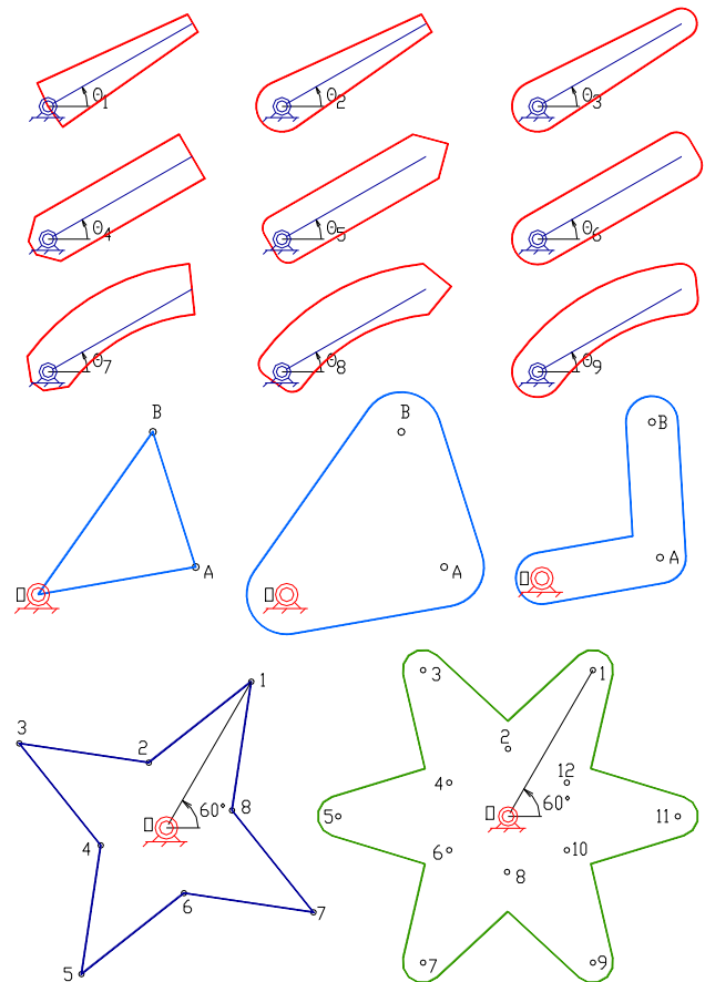
Figure 3: Binary, ternary and polynary shapes generated using LibMec2D subroutines.
