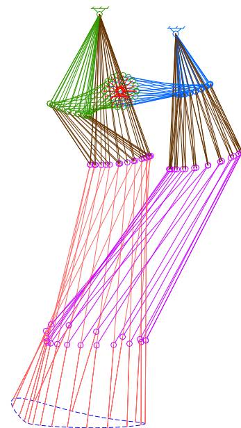
Figure A10: Simulation of a leg mechanism shown as accumulated positions [46].
