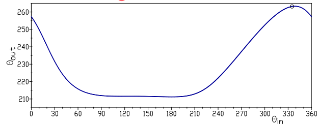
Figure A6: A dwell six-bar linkage and I/O comet plot [1].
