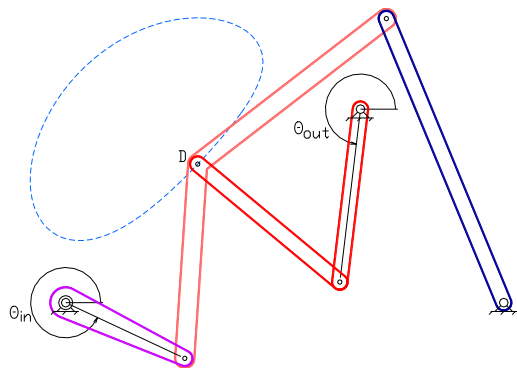
Figure A5: Direct kinematics of a 5R robot [46].
