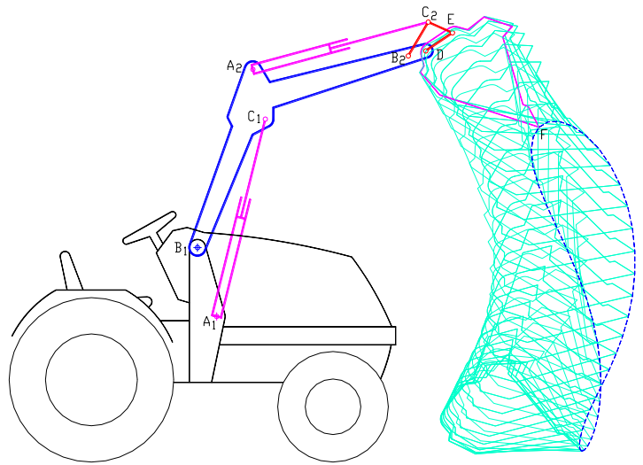
Figure 6: Front loader mechanism that uses two RTRR oscillating slide actuators and one RRR dyad.
